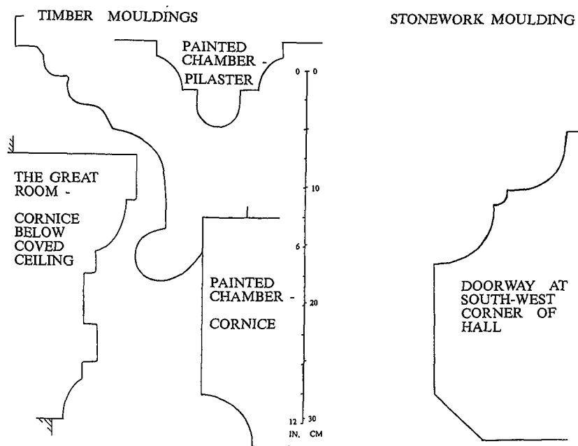
Fig. 6 Ford Place Wrotham: Some examples of Mouldings
